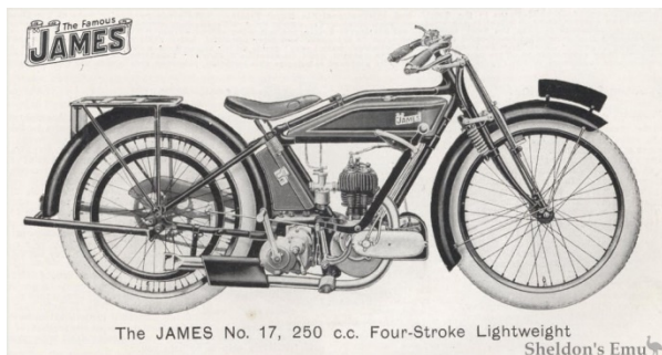
James 1927, 250 cc, four-stroke
